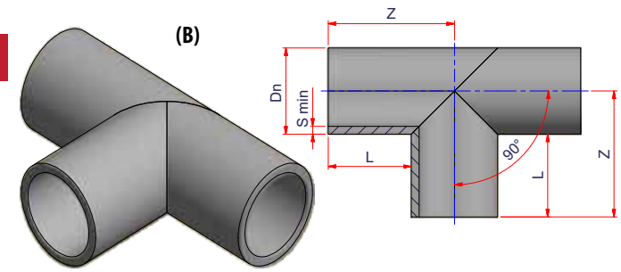
TEE 90° - LONG SPIGOT (SDR 11)
